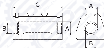
DF (SHORT) DEEP INDENT DIES LF (LONG) DEEP INDENT DIES
