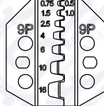
LY-16WF9P dies for wire ferrules end sleeves 0.5-16sqmm 20-6 AWG
