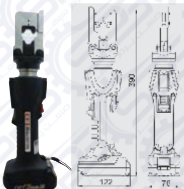
MEPB-185 (18V Li-Ion)
