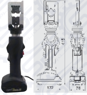
MEPS-240 (18V Li-Ion/ Smart Version)
