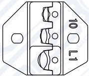
LY-03C Dies for Insulated lugs 0.5-6sqmm 20-10 AWG
