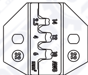
LY-S2 dies for Solar lugs 2.5/4/6sqmm 14/12/10 AWG
