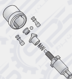
Pin Clutch Mechanism
